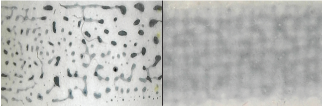
Figure 3. Printed layer of PEDOT:PSS on PDMS recorded under 20x magnification. Left: Without the binding layer, the liquid ink forms droplets and the layer is not conductive. Right: A binding layer printed between PDMS and PEDOT:PSS. The ink forms a connected layer and is conductive. The screen printing mask pattern is visible.
